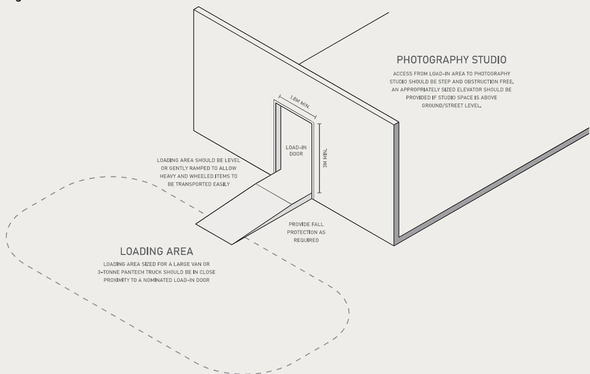
Photography studio – Loading diagram
